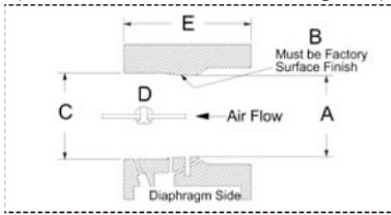
DIAGRAM IS FOR DIMENSIONAL REFERENCE ONLY
